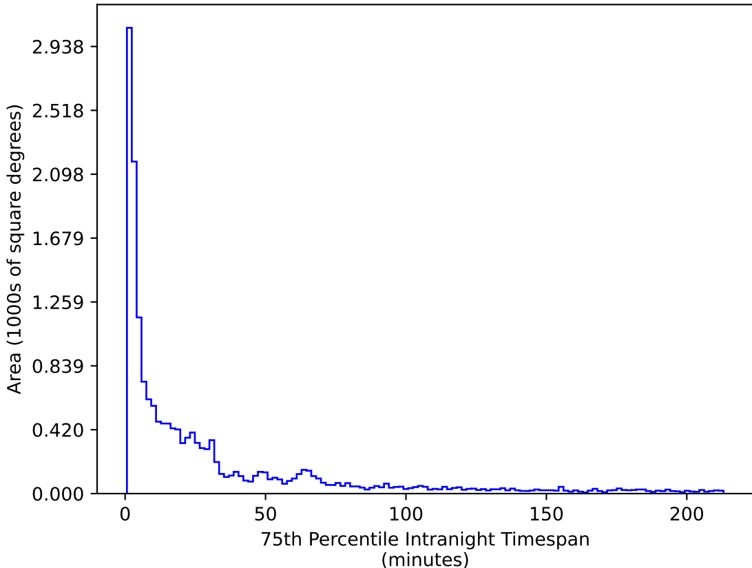
too_ignore_100_4v3.4_10yrs WFD g band: 75th Percentile Intranight Timespan
