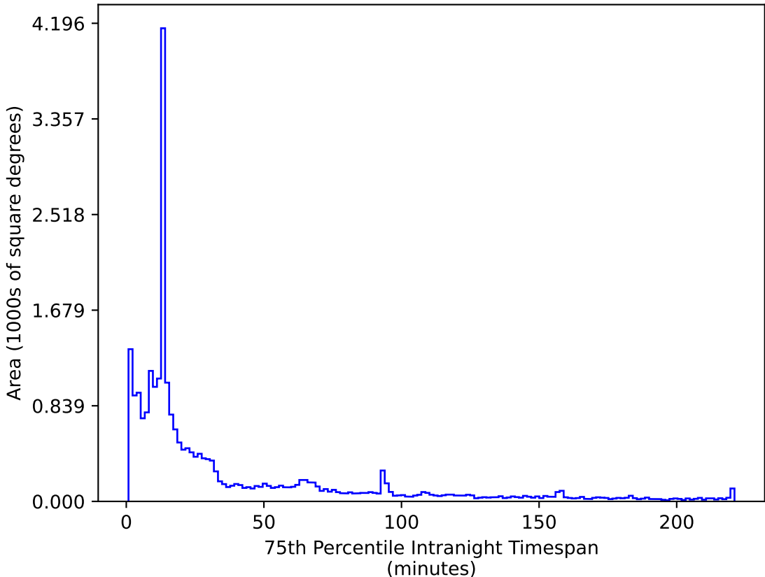
too_ignore_100_4v3.4_10yrs All sky z band: 75th Percentile Intranight Timespan
