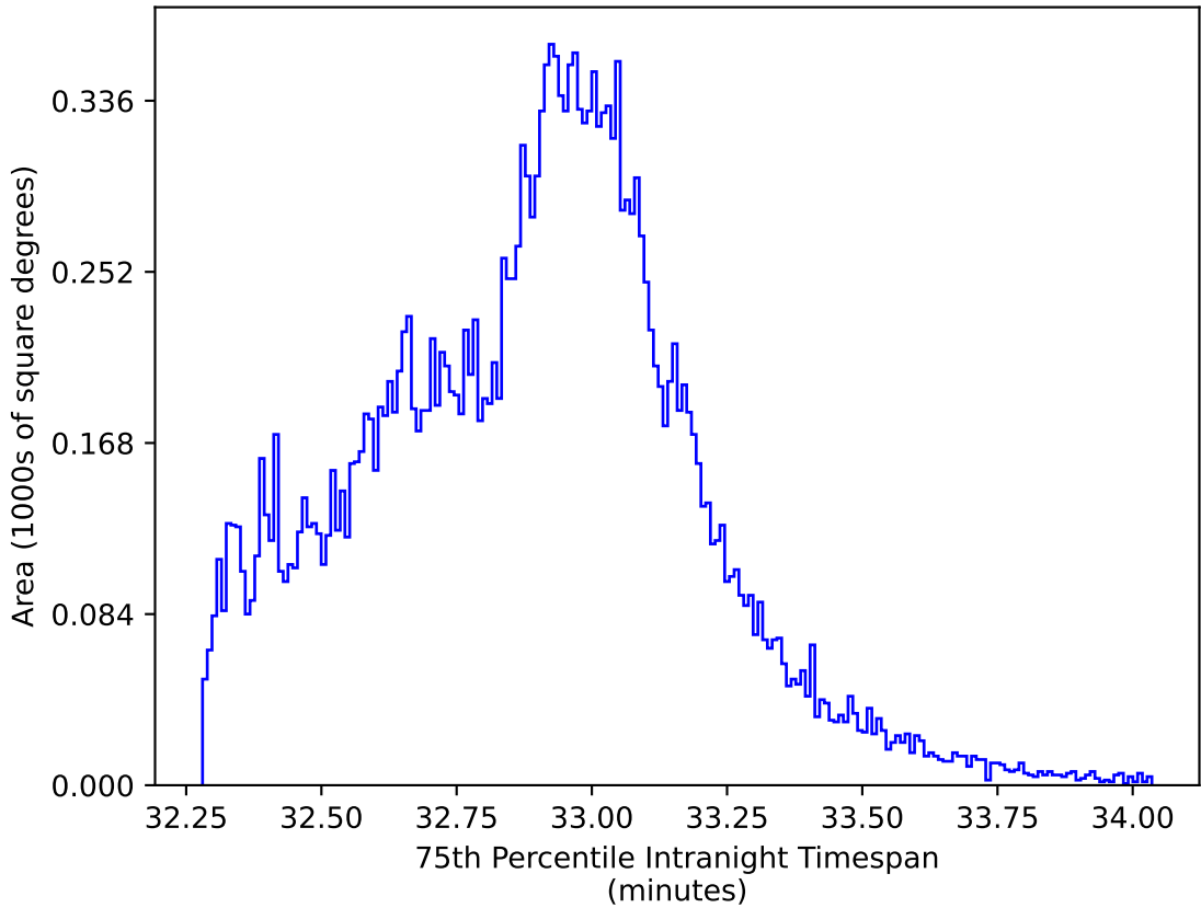
too_ignore_100_4v3.4_10yrs All sky y band: 75th Percentile Intranight Timespan
