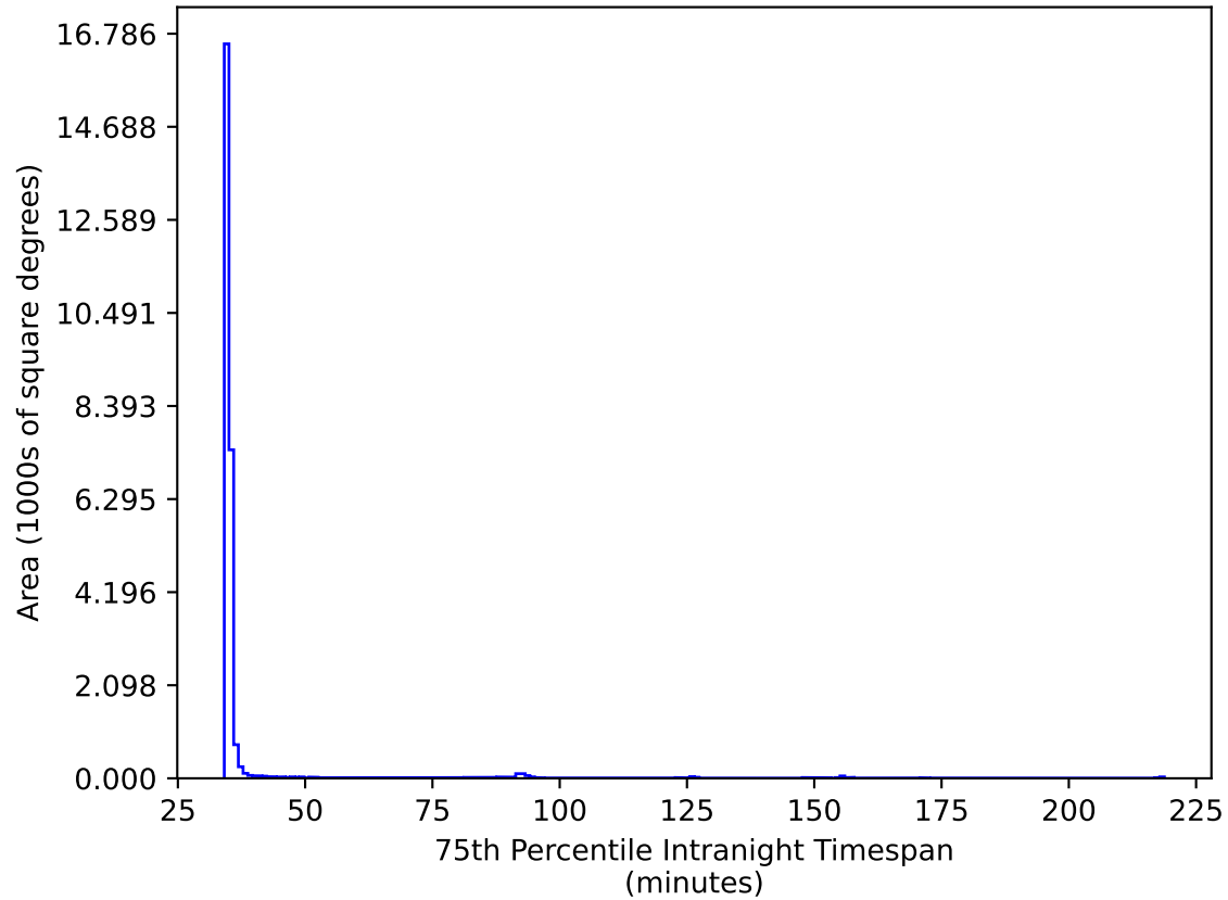
too_ignore_100_4v3.4_10yrs All sky ri bands: 75th Percentile Intranight Timespan
