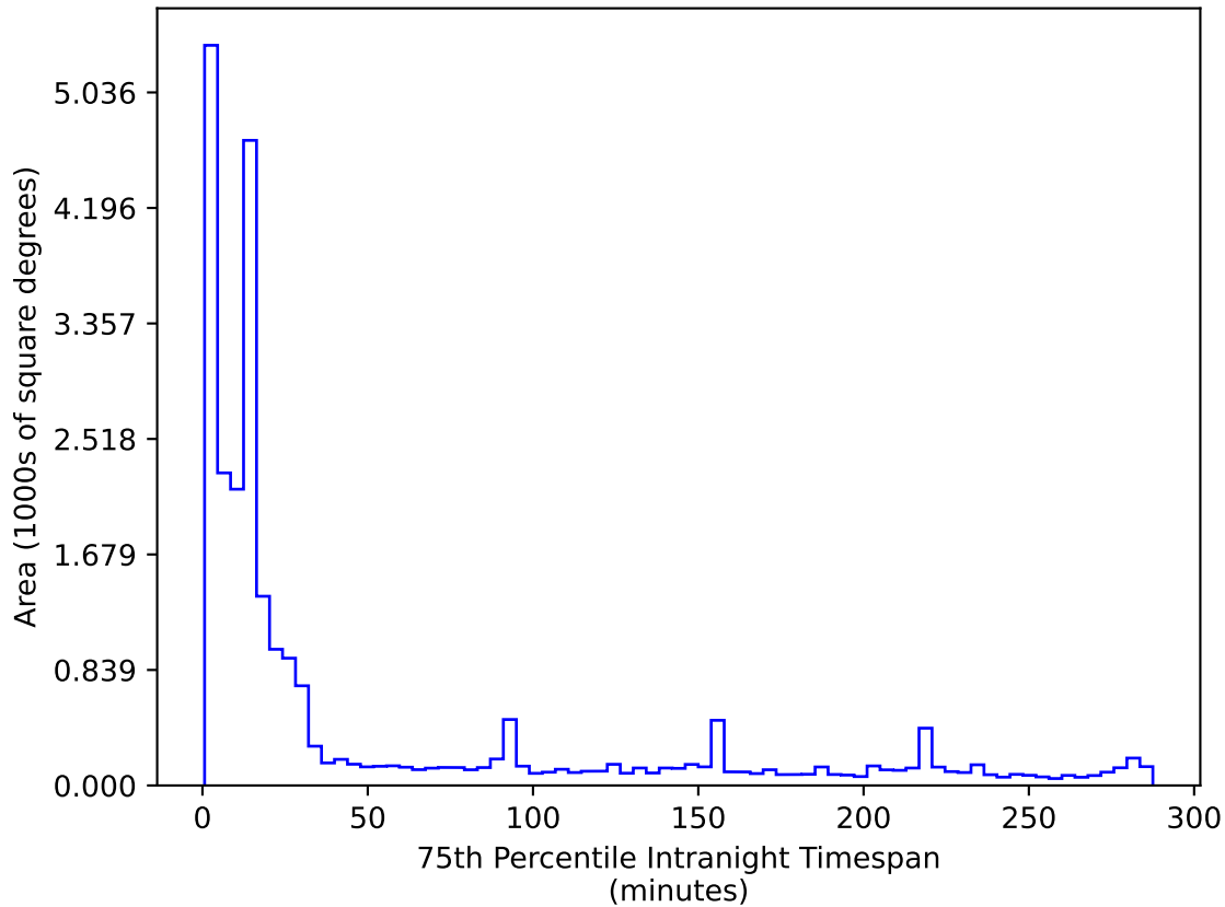
too_ignore_100_4v3.4_10yrs All sky r band: 75th Percentile Intranight Timespan
