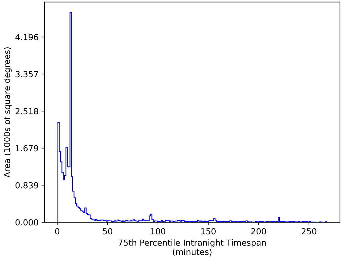
too_ignore_100_4v3.4_10yrs All sky i band: 75th Percentile Intranight Timespan
