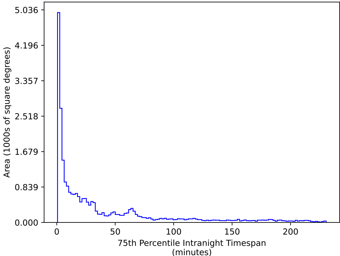
too_ignore_100_4v3.4_10yrs All sky g band: 75th Percentile Intranight Timespan
