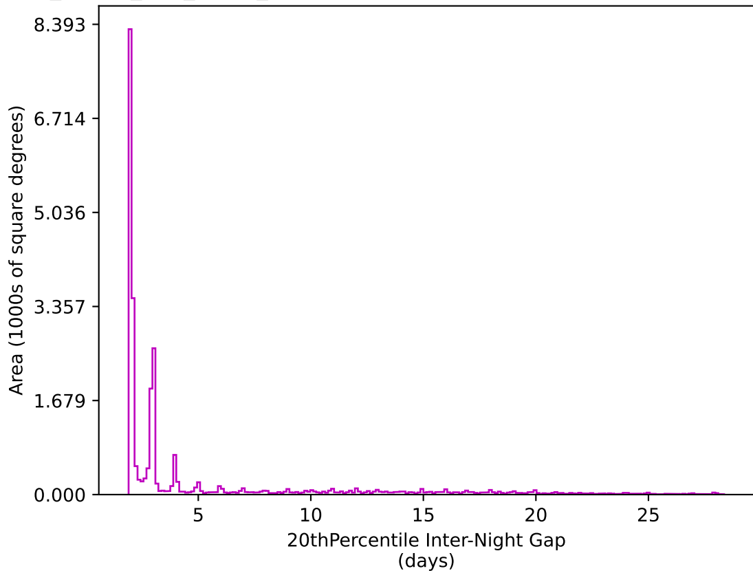
too_ignore_100_4v3.4_10yrs All sky z band: 20thPercentile Inter-Night Gap
