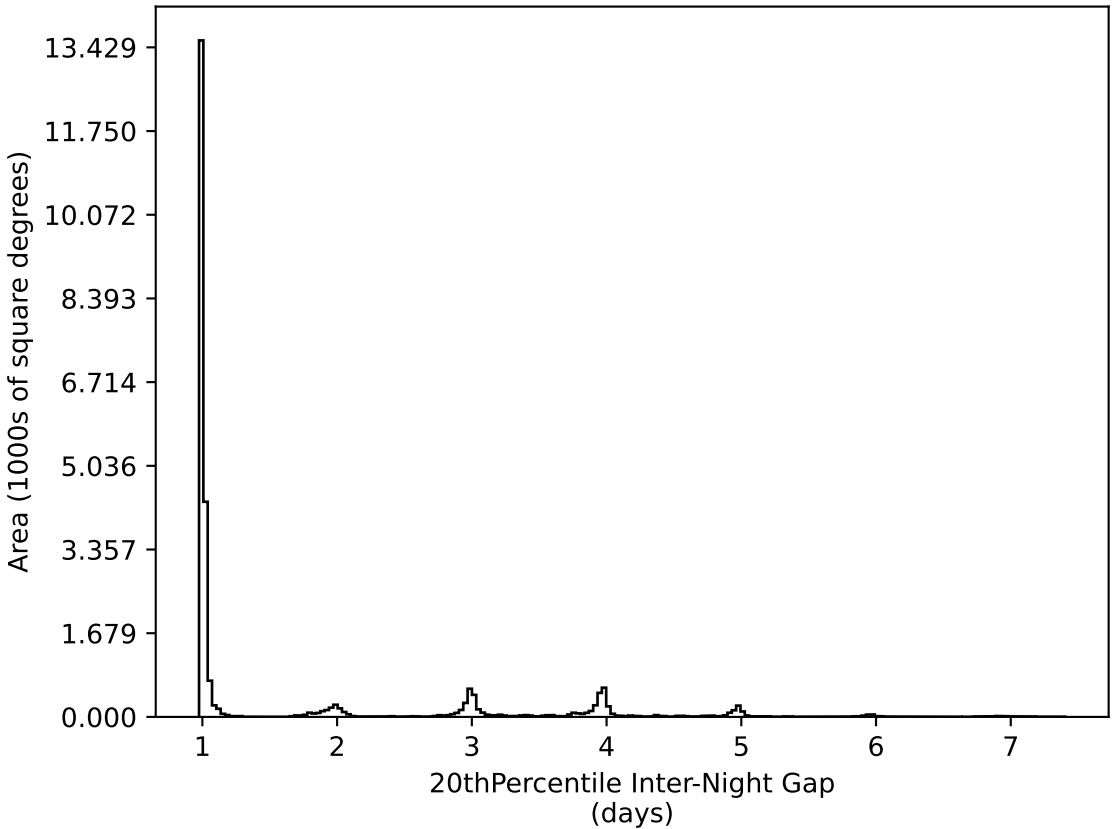
too_ignore_100_4v3.4_10yrs All sky all bands: 20thPercentile Inter-Night Gap
