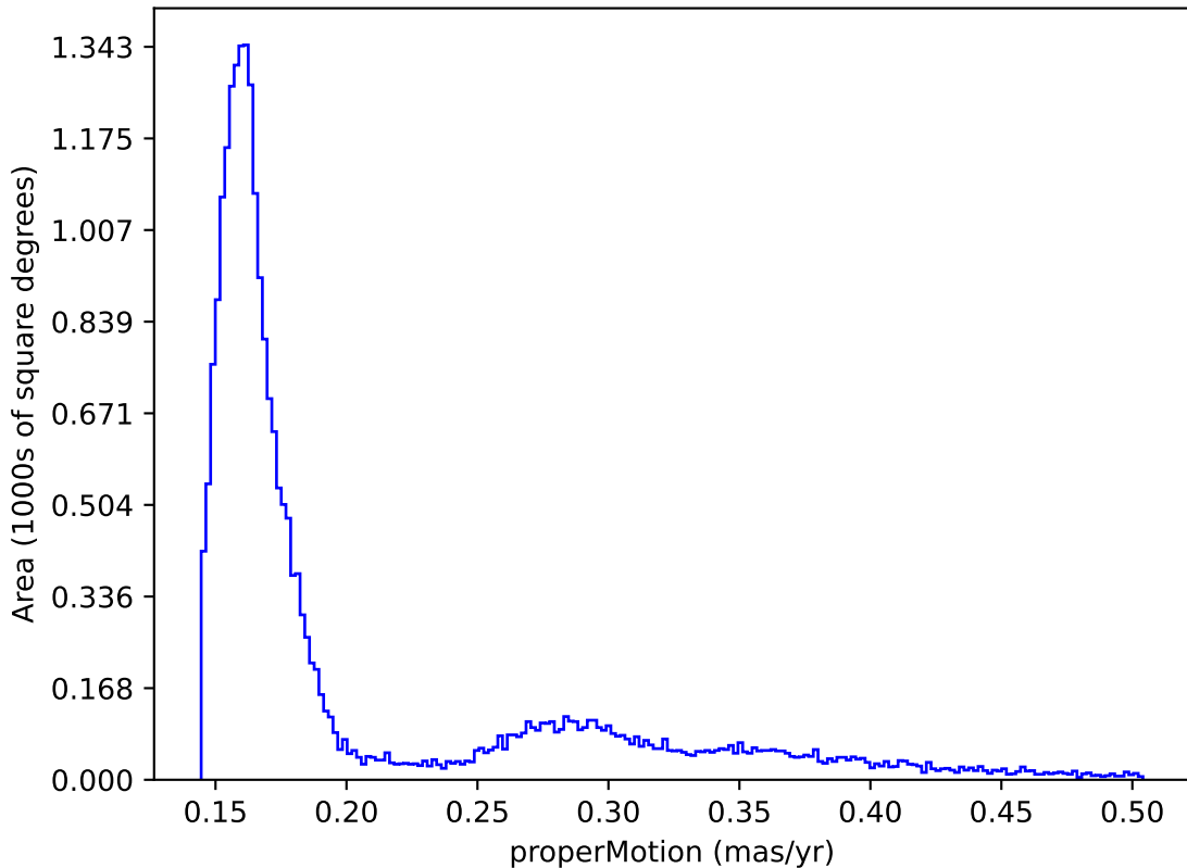
too_ignore_100_4v3.4_10yrs : properMotion
