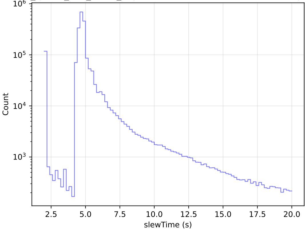
too_ignore_100_4v3.4_10yrs All visits: Zoom Slew Time Histogram
