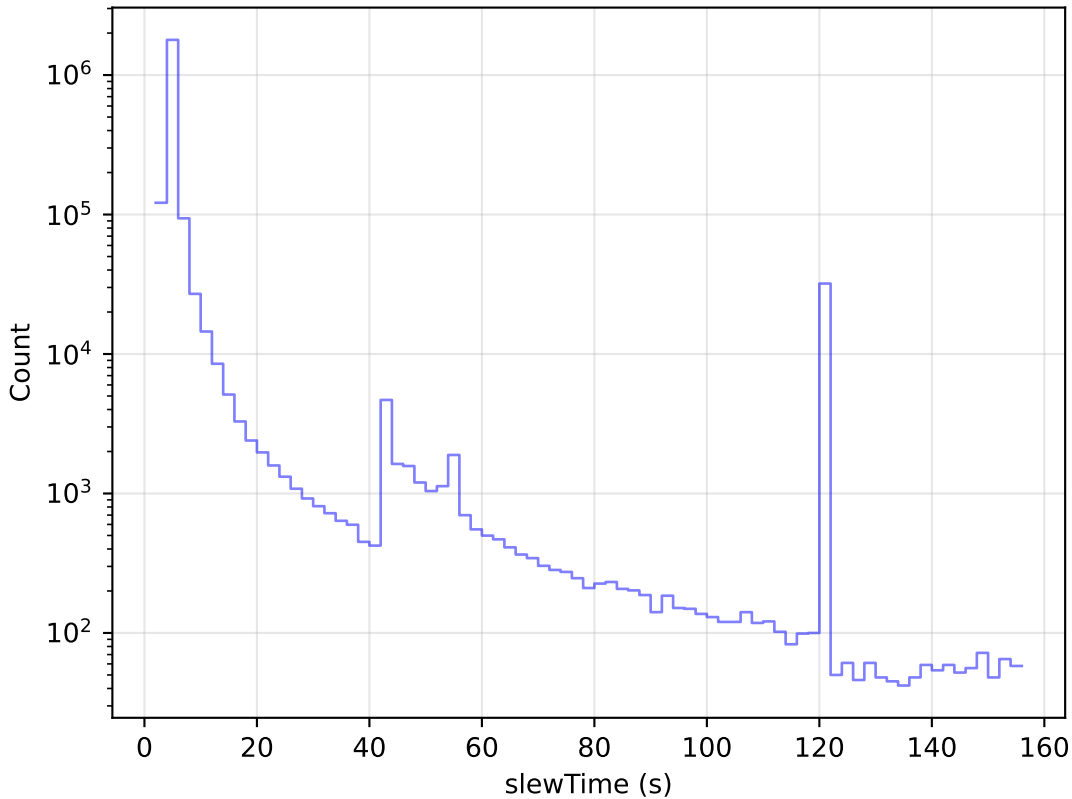
too_ignore_100_4v3.4_10yrs All visits: Slew Time Histogram
