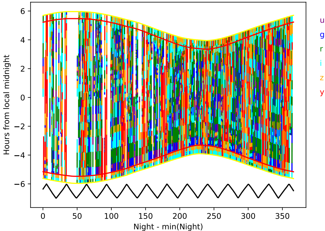
too_ignore_100_4v3.4_10yrs year 6-7: Hourglass
