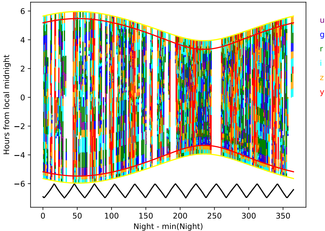
too_ignore_100_4v3.4_10yrs year 5-6: Hourglass
