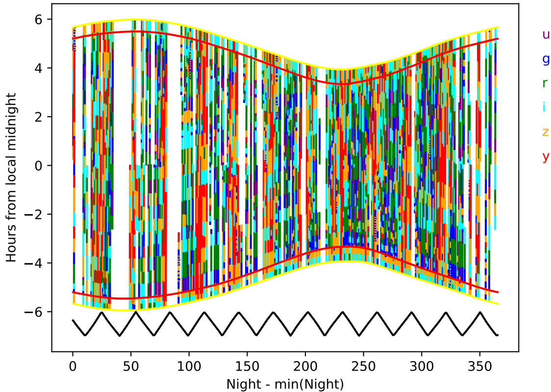
too_ignore_100_4v3.4_10yrs year 4-5: Hourglass
