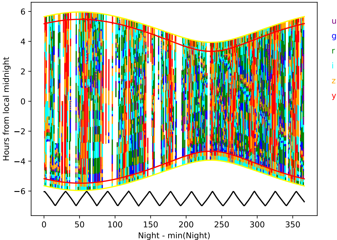
too_ignore_100_4v3.4_10yrs year 1-2: Hourglass
