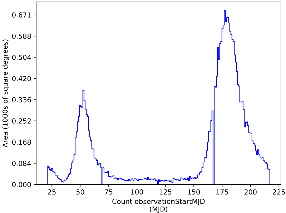
too_ignore_100_4v3.4_10yrs r: Count observationStartMJD
