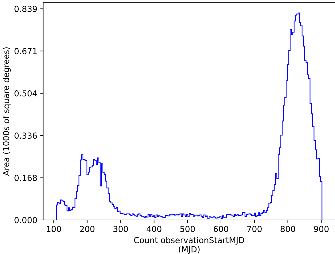
too_ignore_100_4v3.4_10yrs : Count observationStartMJD
