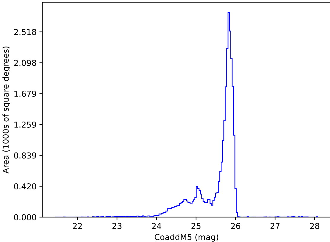
too_ignore_100_4v3.4_10yrs z: CoaddM5
