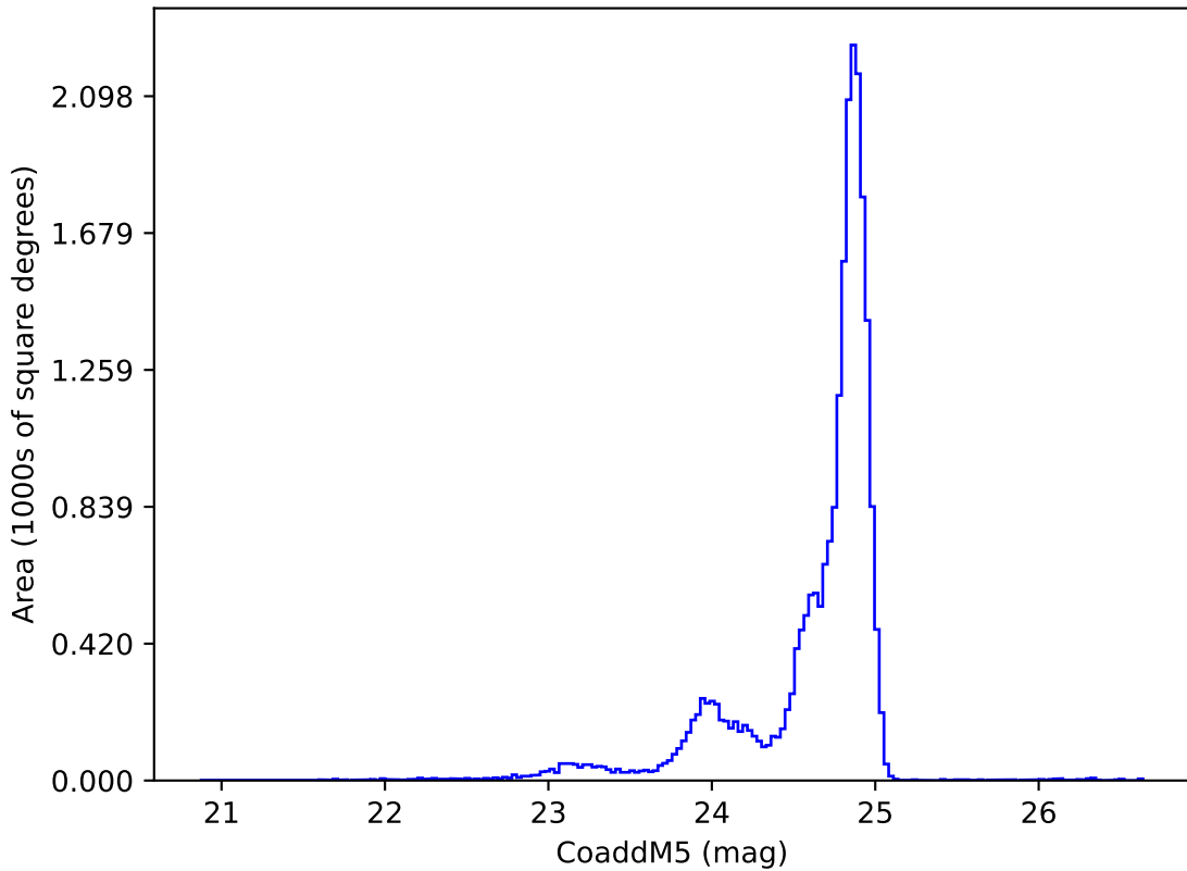
too_ignore_100_4v3.4_10yrs y: CoaddM5
