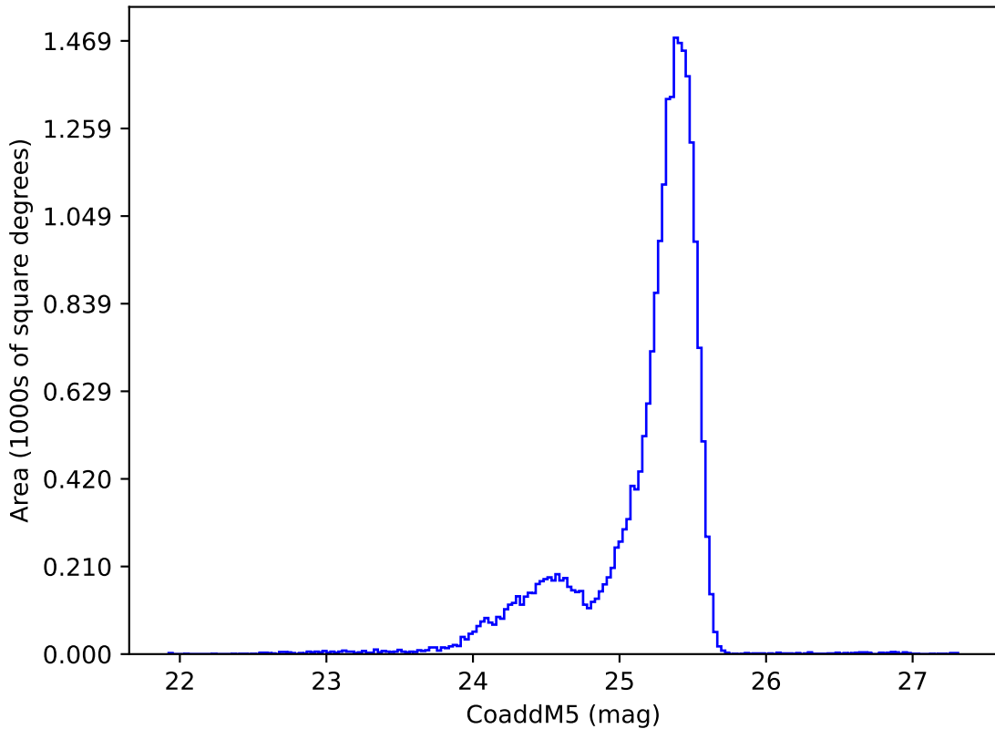
too_ignore_100_4v3.4_10yrs u: CoaddM5
