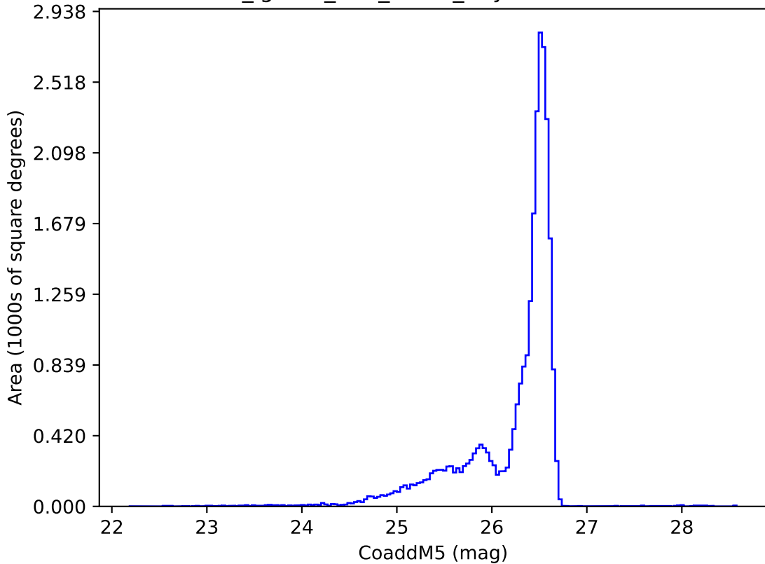
too_ignore_100_4v3.4_10yrs i: CoaddM5
