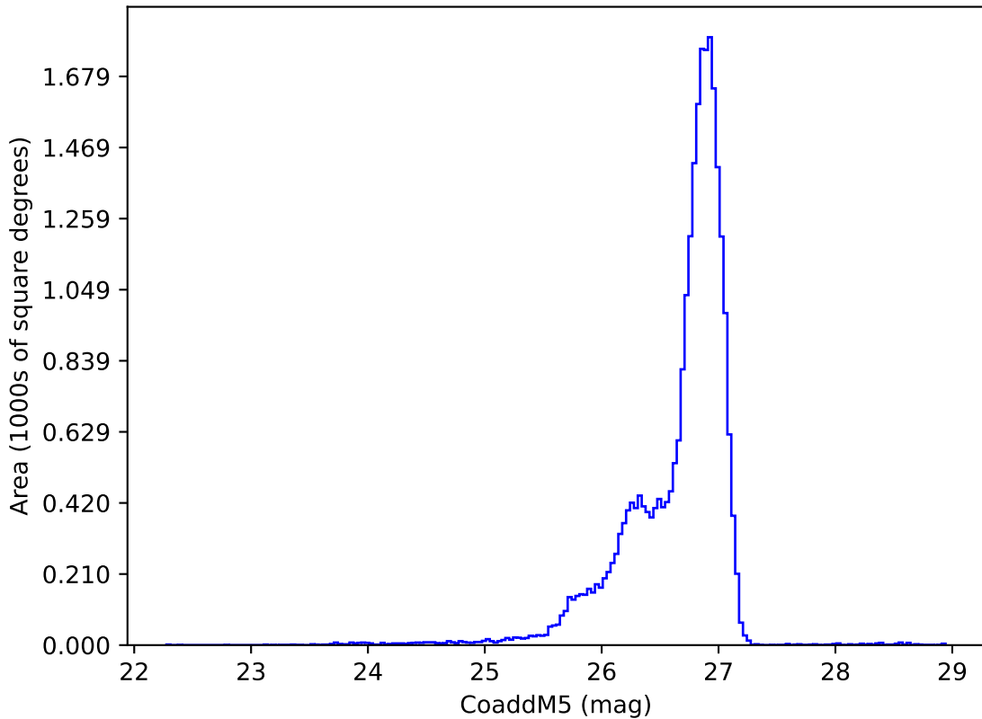
too_ignore_100_4v3.4_10yrs g: CoaddM5
