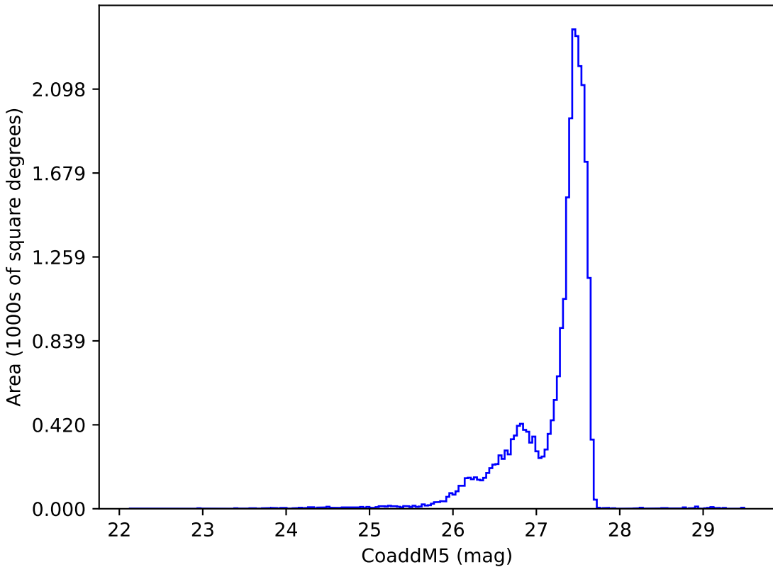
too_ignore_100_4v3.4_10yrs : CoaddM5
