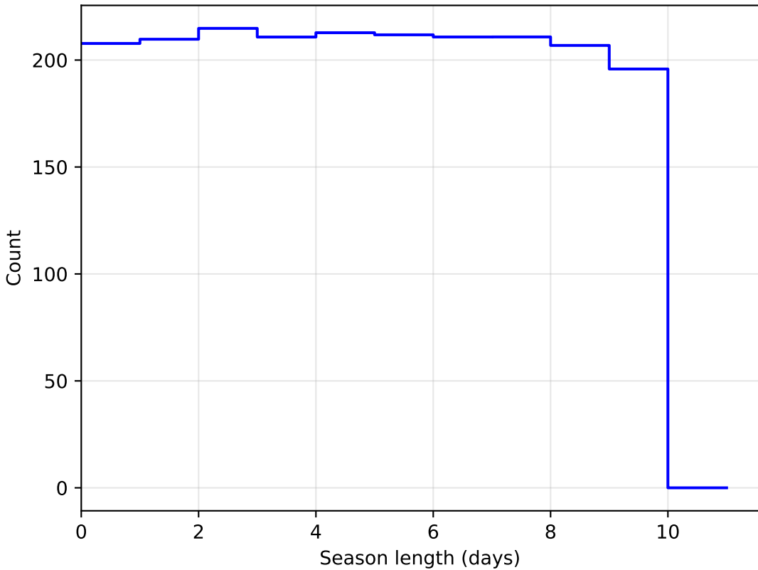
too_ignore_100_4v3.4_10yrs DD:EDFS all bands: SeasonLength
