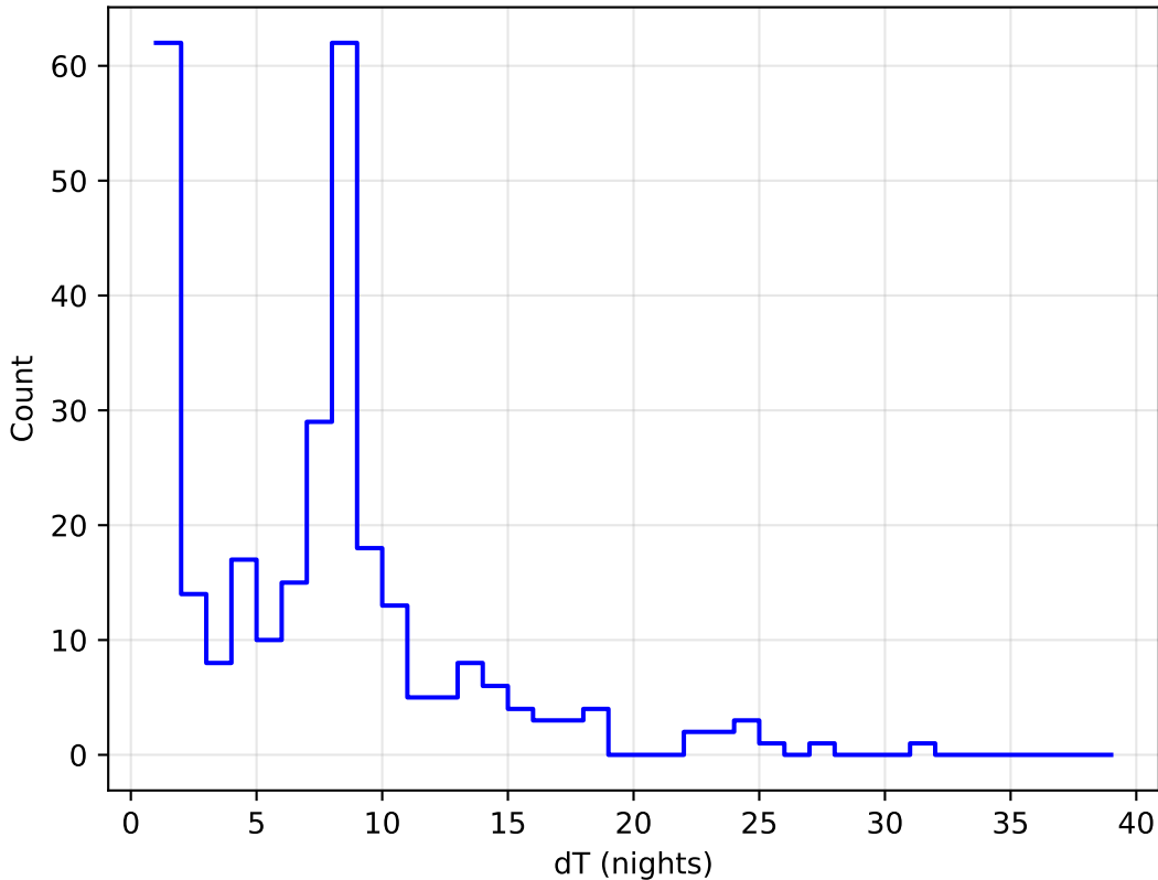
too_ignore_100_4v3.4_10yrs all bands: DD:XMM_LSS Delta Nights Histogram
