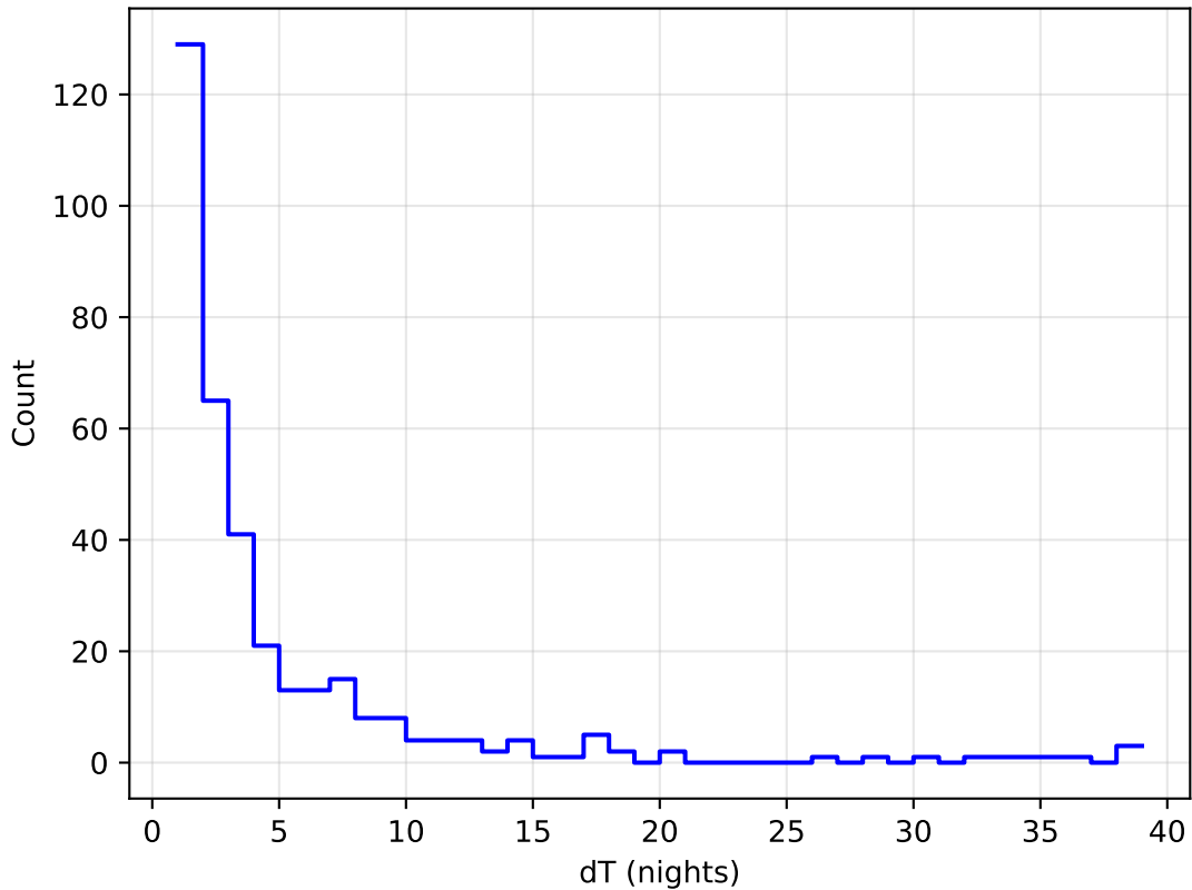
too_ignore_100_4v3.4_10yrs all bands: DD:WFD Delta Nights Histogram
