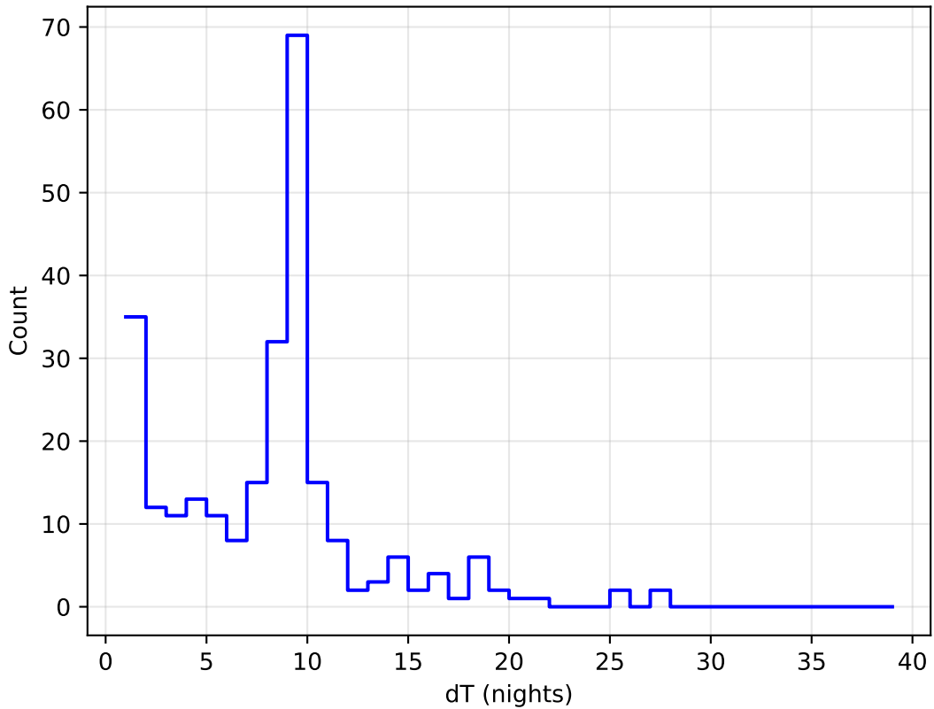
too_ignore_100_4v3.4_10yrs all bands: DD:ELAISS1 Delta Nights Histogram
