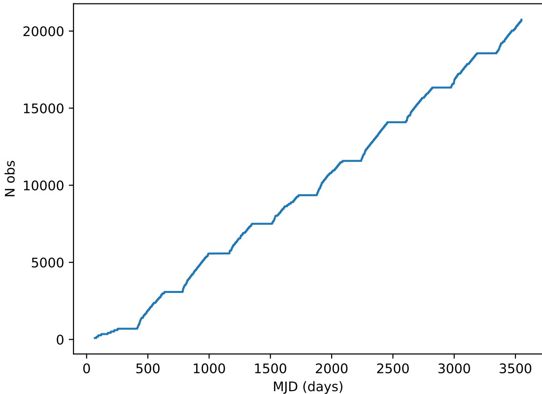
too_ignore_100_4v3.4_10yrs all bands: DD:ELAISS1 Cumulative NVisits
