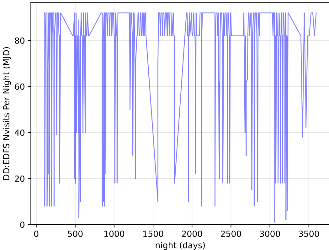
too_ignore_100_4v3.4_10yrs all bands: DD:EDFS Nvisits Per Night
