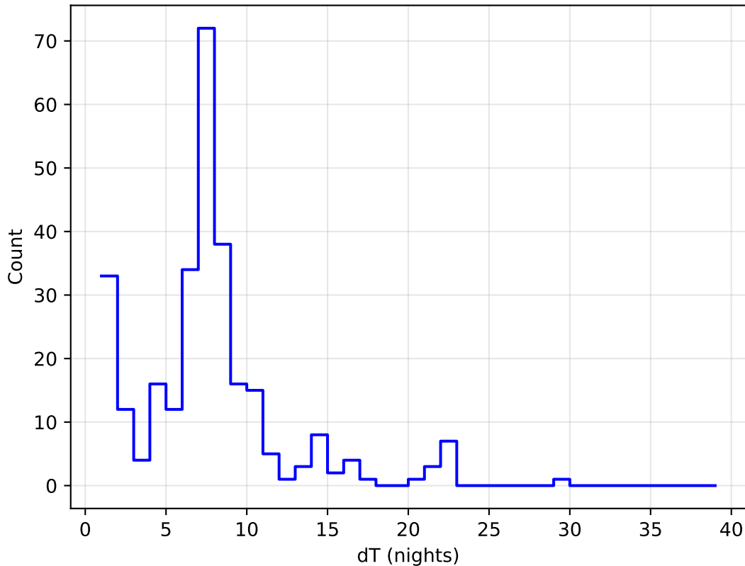
too_ignore_100_4v3.4_10yrs all bands: DD:EDFS Delta Nights Histogram
