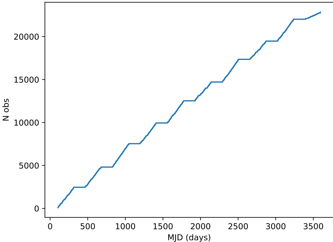
too_ignore_100_4v3.4_10yrs all bands: DD:EDFS Cumulative NVisits
