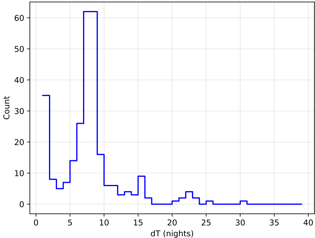
too_ignore_100_4v3.4_10yrs all bands: DD:ECDFS Delta Nights Histogram
