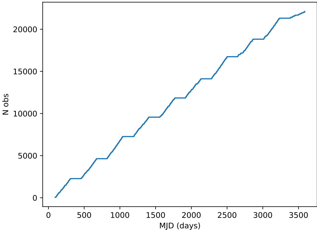
too_ignore_100_4v3.4_10yrs all bands: DD:ECDFS Cumulative NVisits
