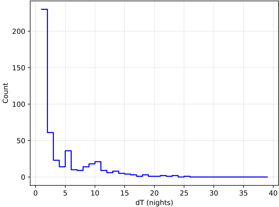
too_ignore_100_4v3.4_10yrs all bands: DD: COSMOS Delta Nights Histogram
