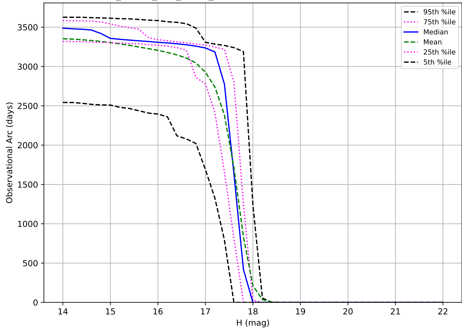
too_ignore_100_1v3.4_10yrs: Observational Arc Length Trojan
