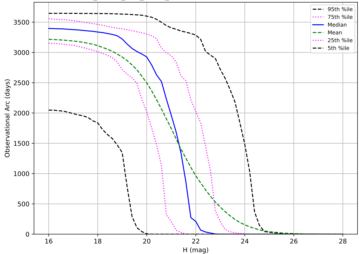
too_ignore_100_1v3.4_10yrs: Observational Arc Length PHA
