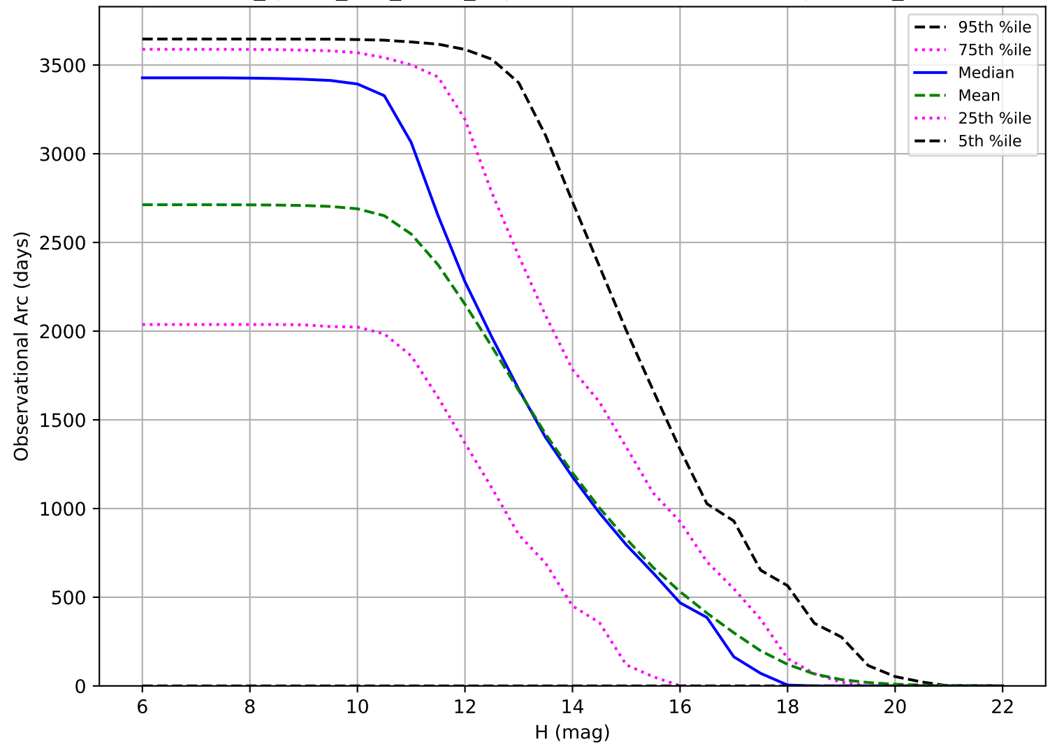
too_ignore_100_1v3.4_10yrs: Observational Arc Length OCC_r5
