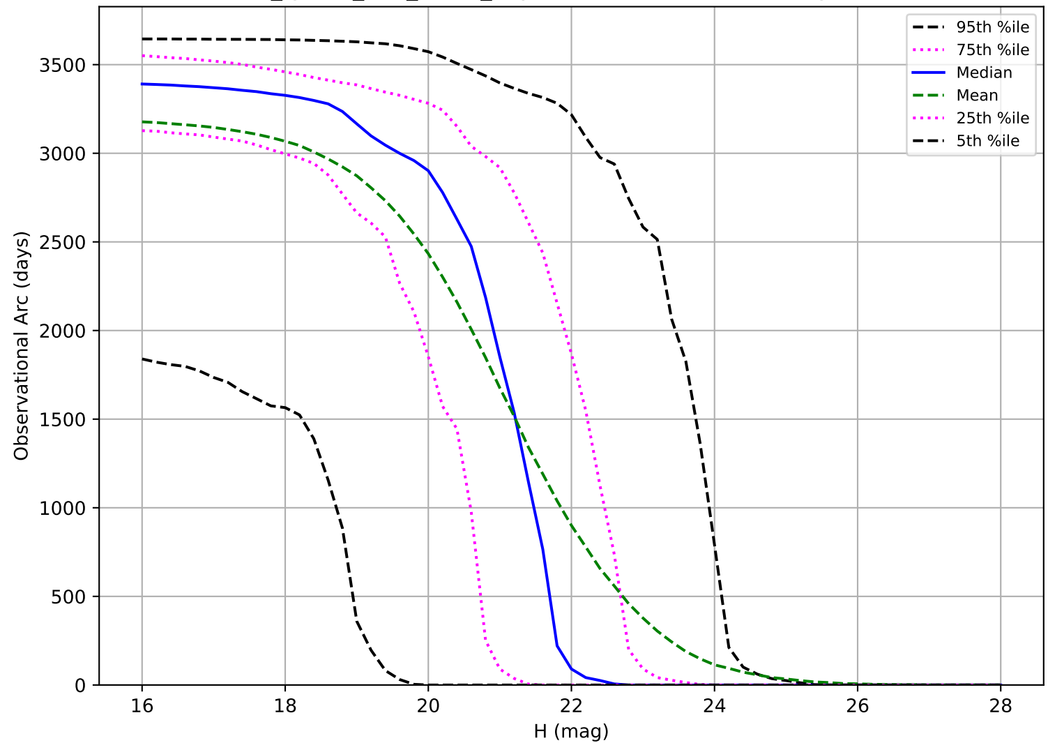
too_ignore_100_1v3.4_10yrs: Observational Arc Length NEO
