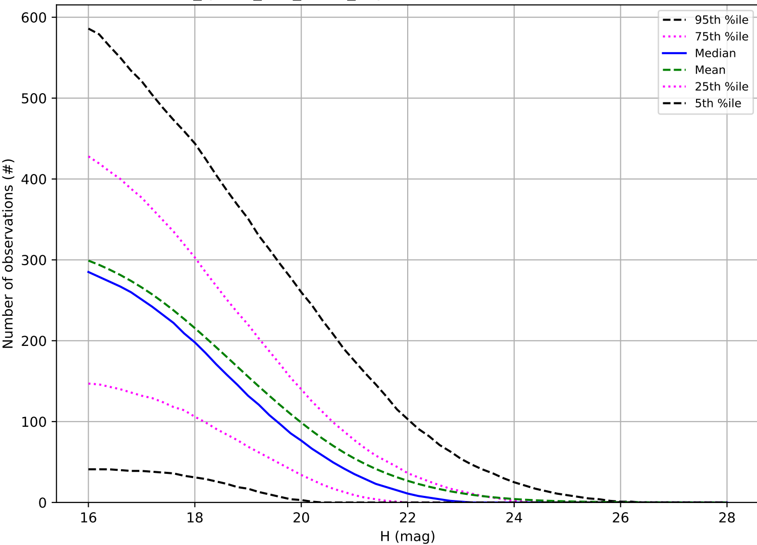
too_ignore_100_1v3.4_10yrs: Number of observations PHA
