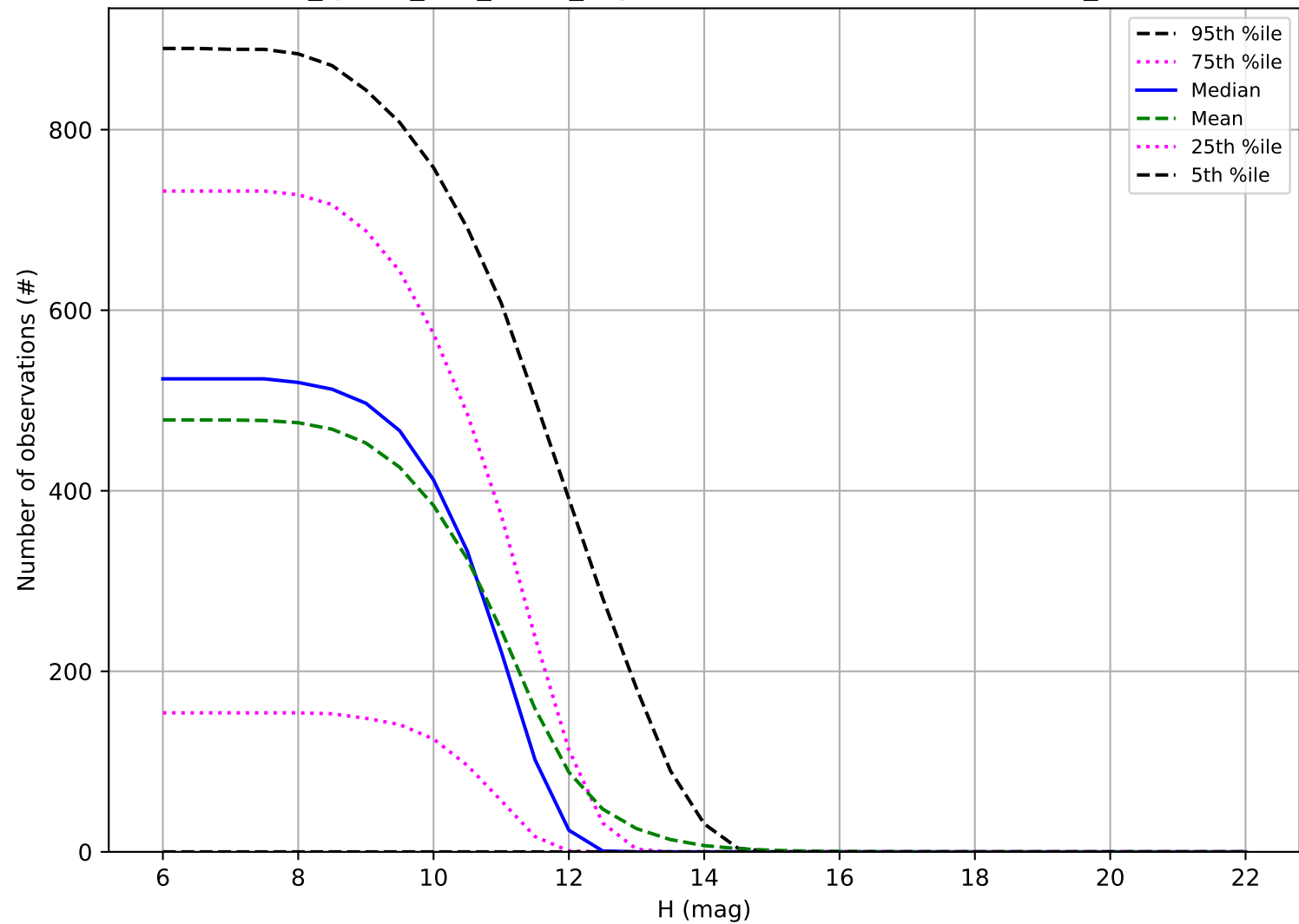
too_ignore_100_1v3.4_10yrs: Number of observations OCC_r20
