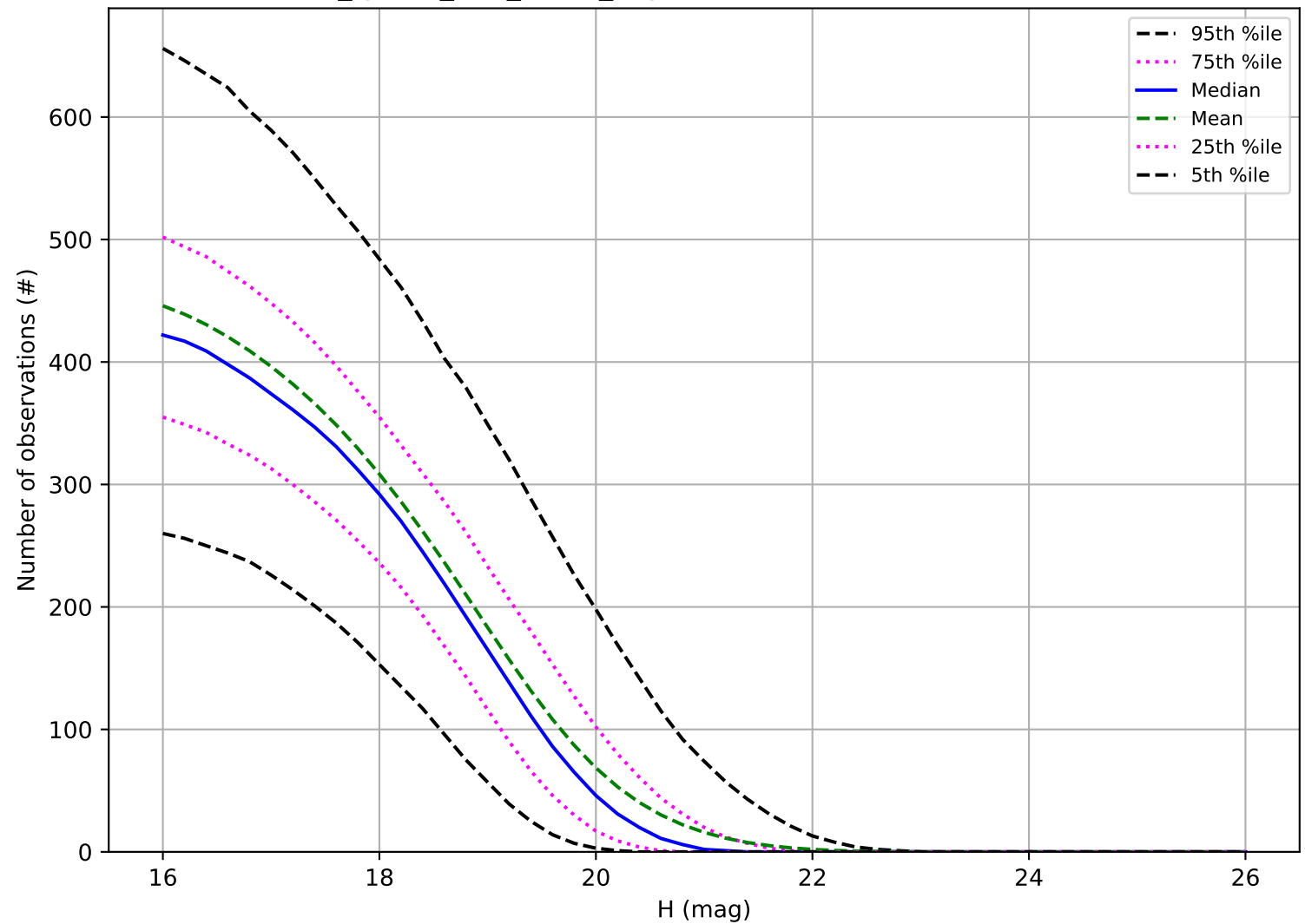
too_ignore_100_1v3.4_10yrs: Number of observations MBA
