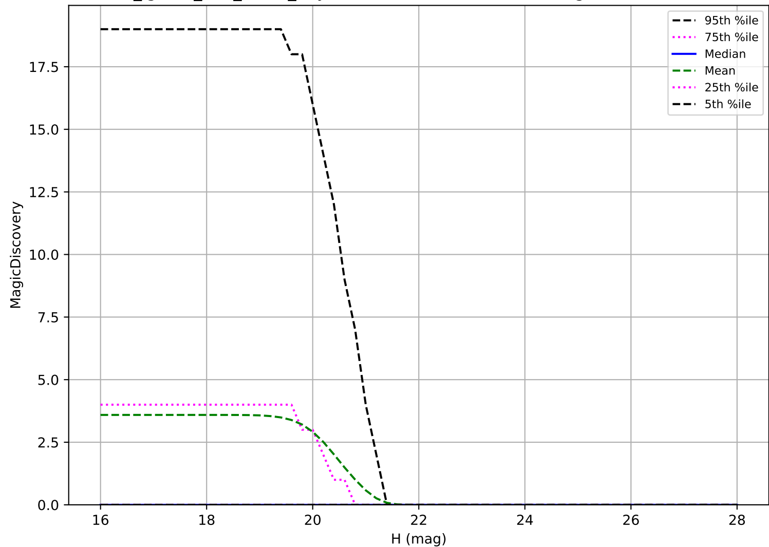
too_ignore_100_1v3.4_10yrs: Vatira 6 detections in 60 nights detection loss
