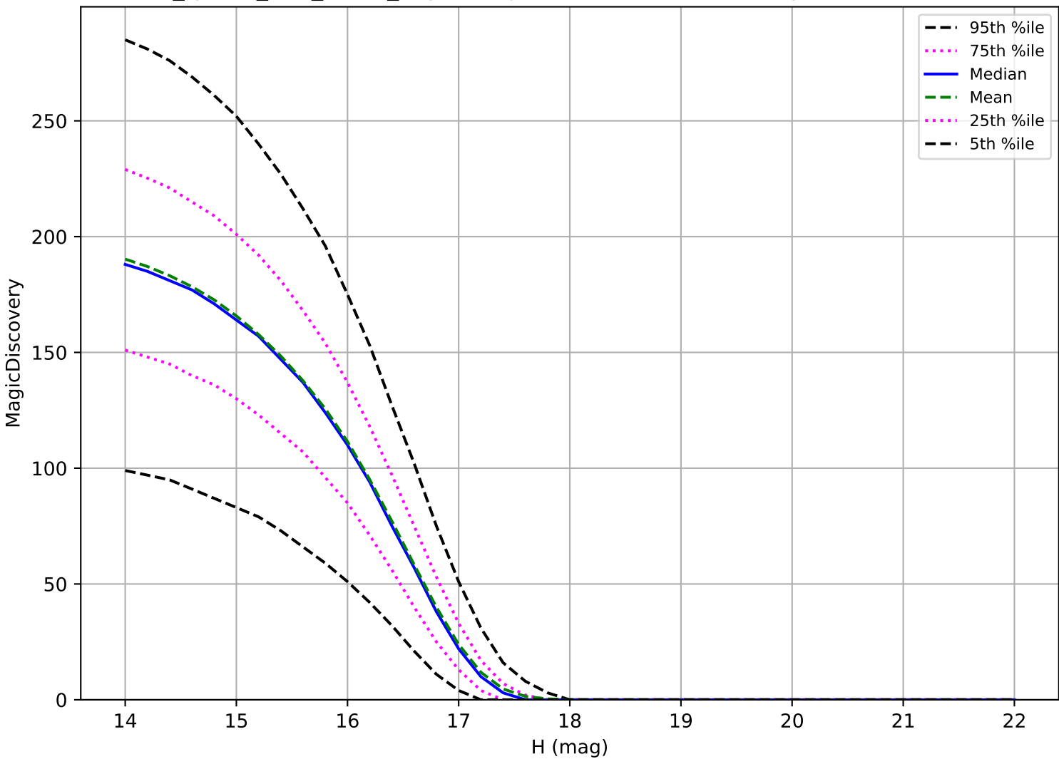
too_ignore_100_1v3.4_10yrs: Trojan 6 detections in 60 nights detection loss
