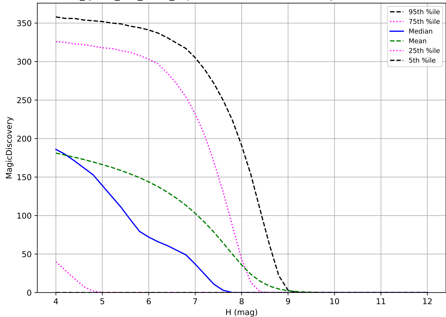
too_ignore_100_1v3.4_10yrs: TNO 6 detections in 60 nights detection loss
