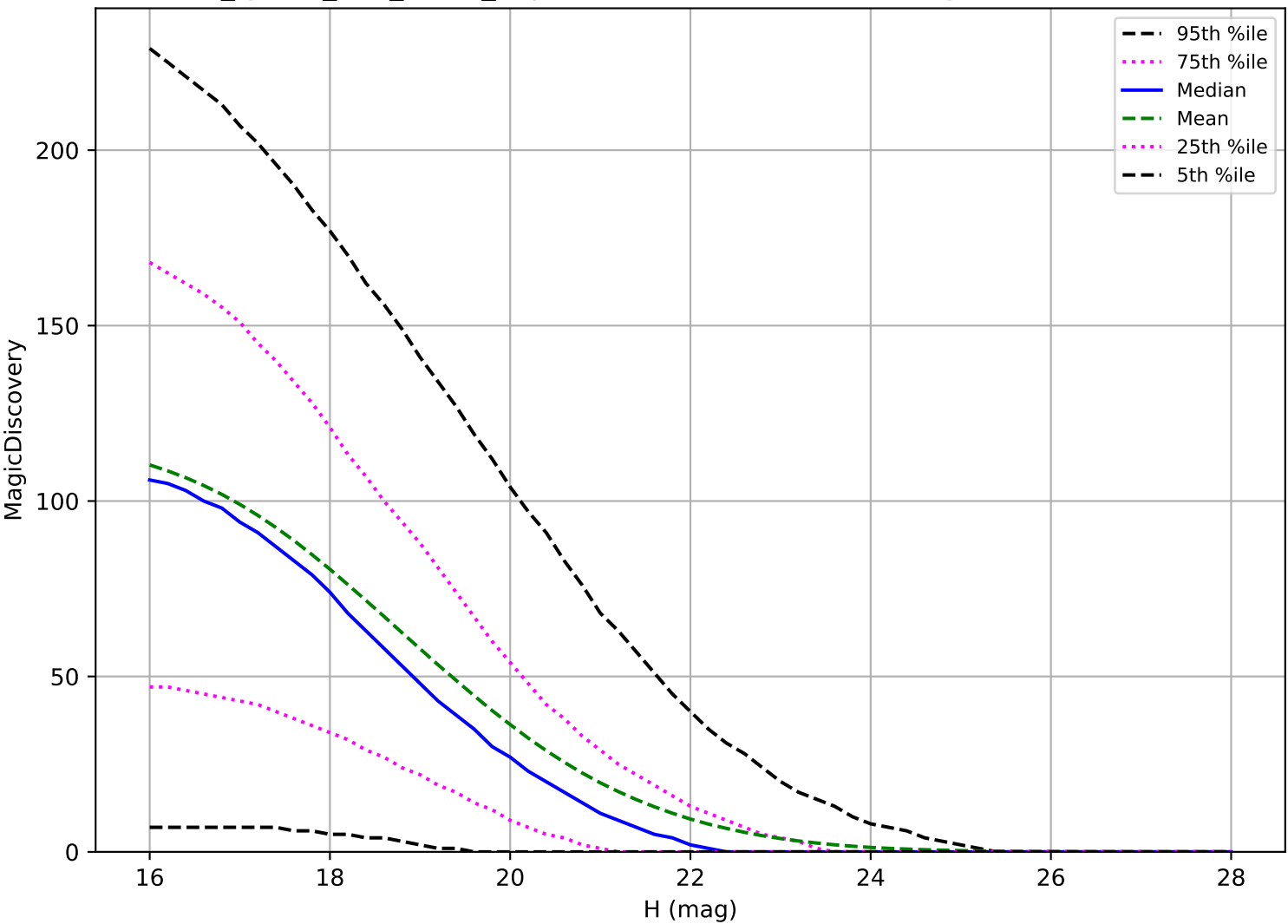
too_ignore_100_1v3.4_10yrs: PHA 6 detections in 60 nights detection loss
