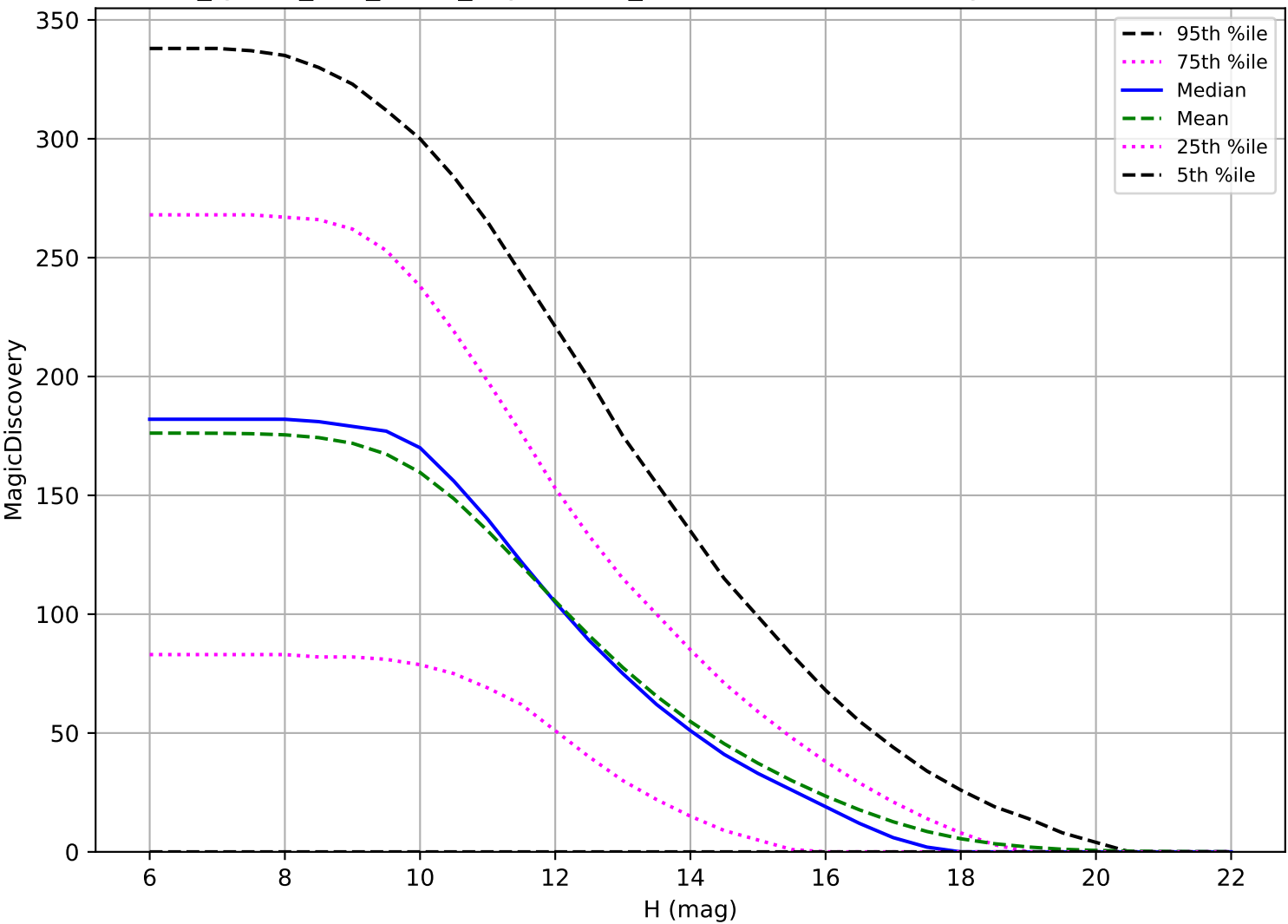
too_ignore_100_1v3.4_10yrs: OCC_r5 6 detections in 60 nights detection loss
