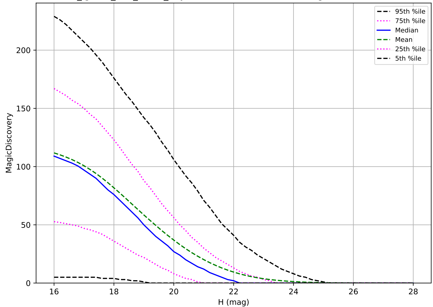
too_ignore_100_1v3.4_10yrs: NEO 6 detections in 60 nights detection loss
