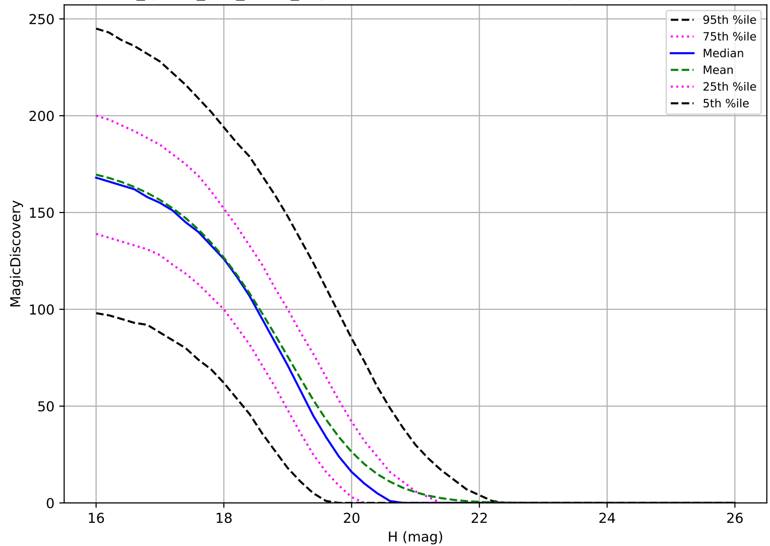
too_ignore_100_1v3.4_10yrs: MBA 6 detections in 60 nights detection loss
