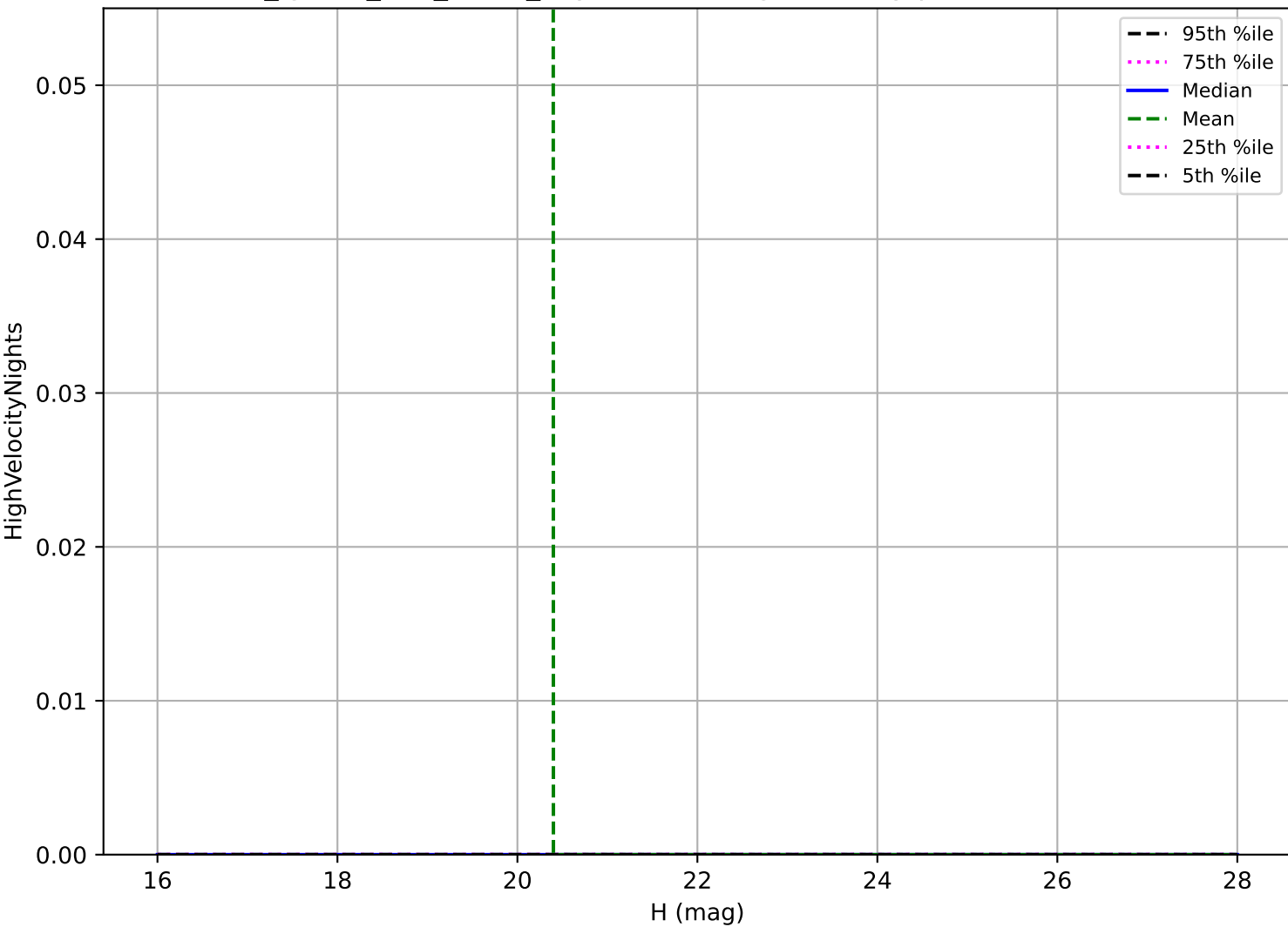
too_ignore_100_1v3.4_10yrs: Vatira High velocity pair detection loss
